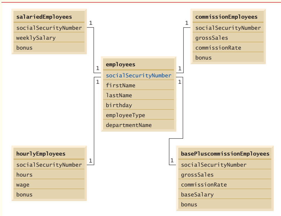
Fig. 24.33 | Table relationships in the employees database.
